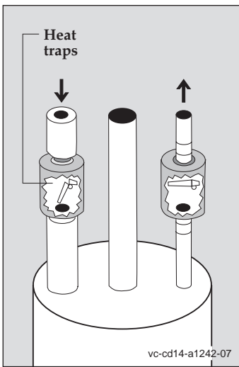
Heat traps, or one-way valves, can control the flow of water into and out of your storage tank.
